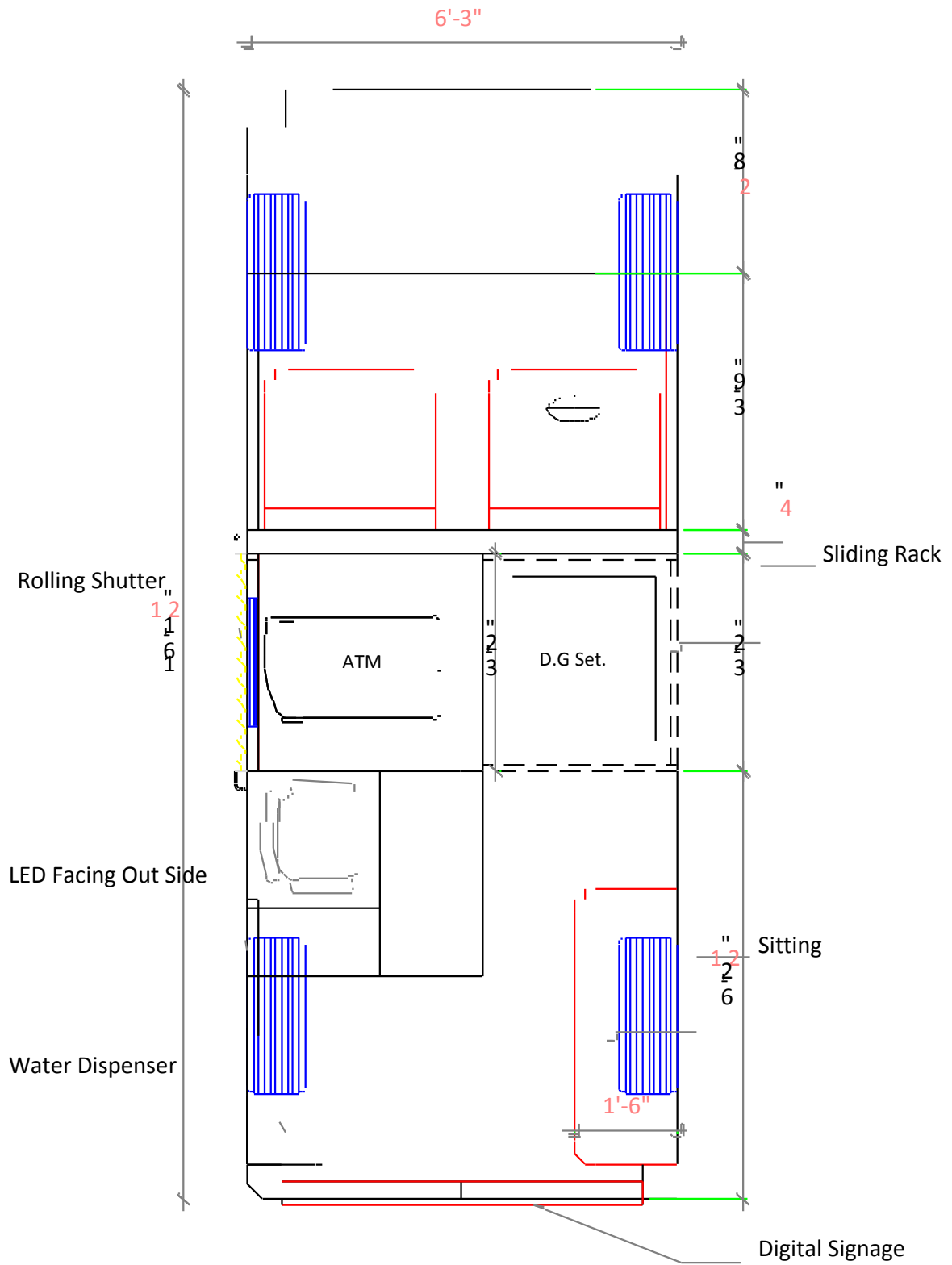
Mobile ATM Layout Plan Winger Cargo
